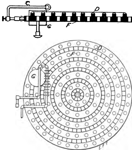
FIG. 216.—Plan and Sectional Elevation of the White Burner.
